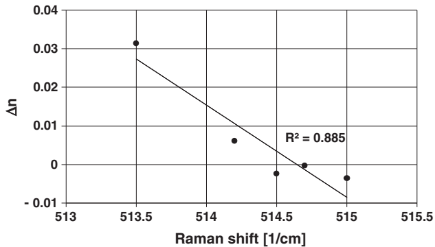
Fig. 3. Comparison of nonlinear refraction with Raman shift of the LO phonon in Si.
