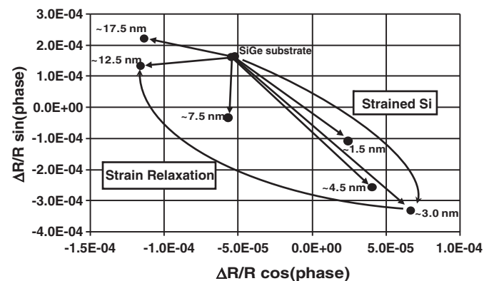
Fig. 2. Laser PR signal from strained silicon on silicon-germanium substrates (after Ref. 10).
