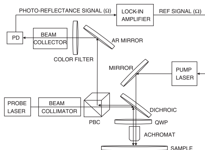
Fig. 1. Schematic of laser PR apparatus.
