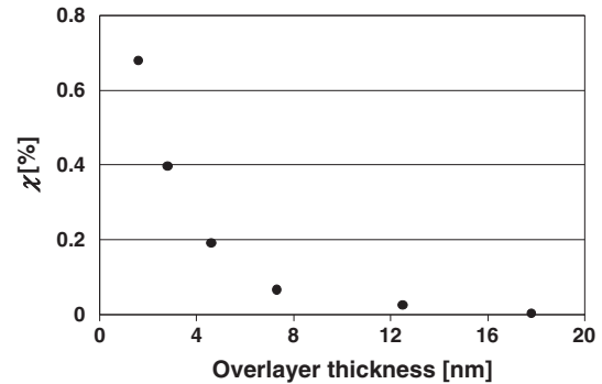
Fig. 4. Strain in silicon overlayers derived from laser PR measurements.
